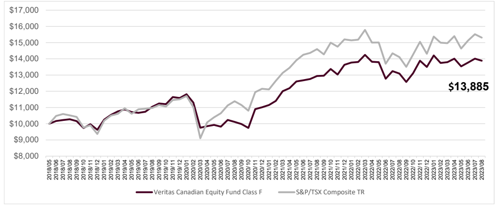
Growth of $10,000 (since inception date)
